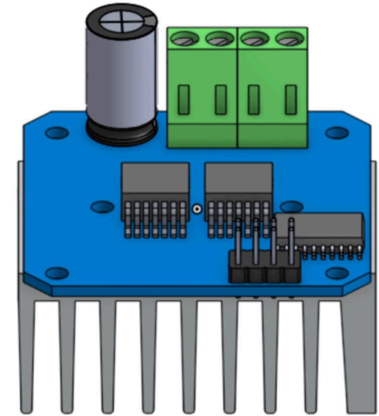
Driver de motor (BTS7960 43A)
